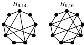
Fig. 1. Eulerian Graphs of order 9 and size 14, 16.
