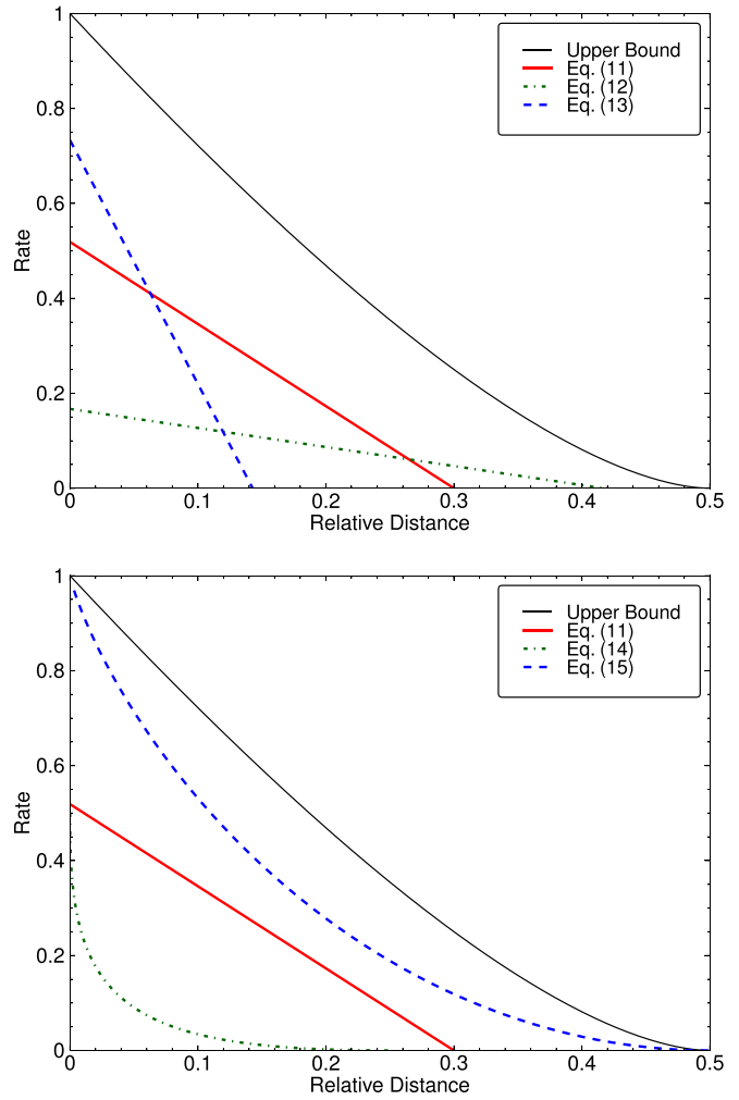
Fig. 3. Upper and lower bounds for \omega = 1/2 .
