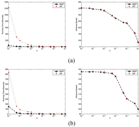
Fig. 4. Running time and influence spread on Wiki for different \theta ( T = 10 , K = 50 , Time Constrained Version). (a) Poisson delay distribution. (b) Geometric delay distribution.
