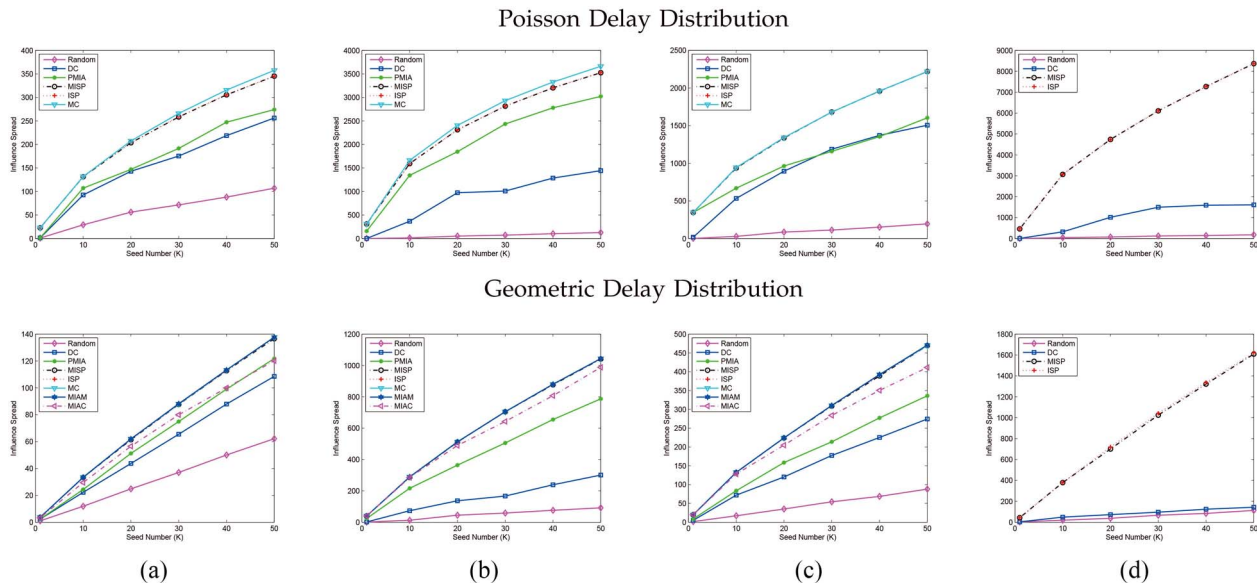
Fig. 6. Influence spread on four real world social networks for different values of K ( T = 10 , Time Constrained Version). (a) Wiki. (b) Epinions. (c) Slashdot. (d) LiveJournal.
