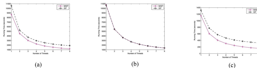
Fig. 11. Running time on Livejournal with different number of threads ( K = 50 ). (a) Poisson Delay Distribution, T = 10 ). (b) Geometric Delay Distribution, T = 10 ). (c) Conventional Version.
