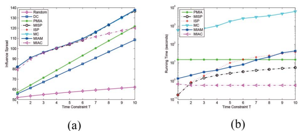
Fig. 10. Results on Wiki with different T ( K = 50 ). (a) Influence Spread. (b) Running Time.
