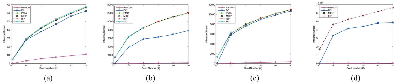
Fig. 7. Influence spread on four real world social networks for different values of K (Conventional Version). (a) Wiki. (b) Epinions. (c) Slashdot. (d) LiveJournal.
