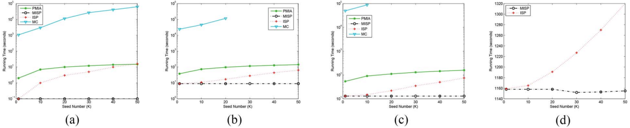
Fig. 9. Running time on four real world social networks for different values of K (Conventional Version). (a) Wiki. (b) Epinions. (c) Slashdot. (d) LiveJournal.
