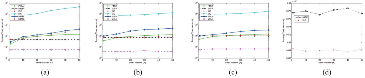
Fig. 8. Running time on four real world social networks for different values of K ( T = 10 , Time Constrained Version). (a) Wiki. (b) Epinions. (c) Slashdot. (d) LiveJournal.
