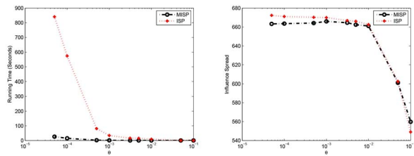
Fig. 5. Running time and influence spread on Wiki for different \theta ( K = 50 , Conventional Version).
