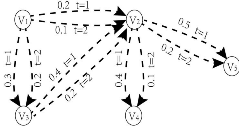
Fig. 2. Logically augmented multigraph with T = 2 .
