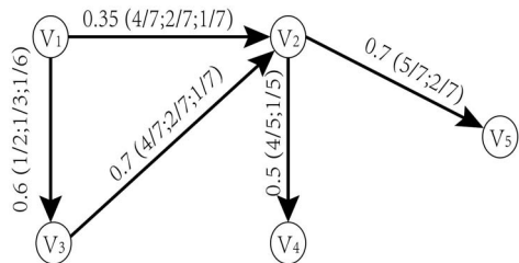
Fig. 1. Example illustrating the time constrained influence maximization.
